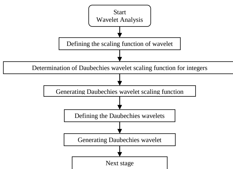
Fig. 4. Schematic of a first stage of the algorithm.
