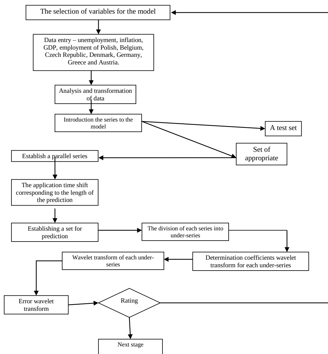
Fig. 5. Schematic of the second stage of the algorithm.
